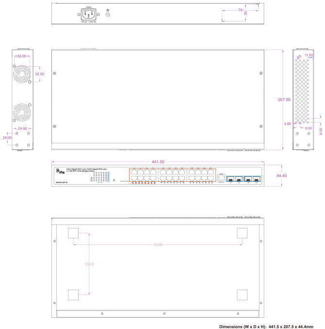
Dimensions (W x D x H): 441.5 x 207.5 x 44.4mm
