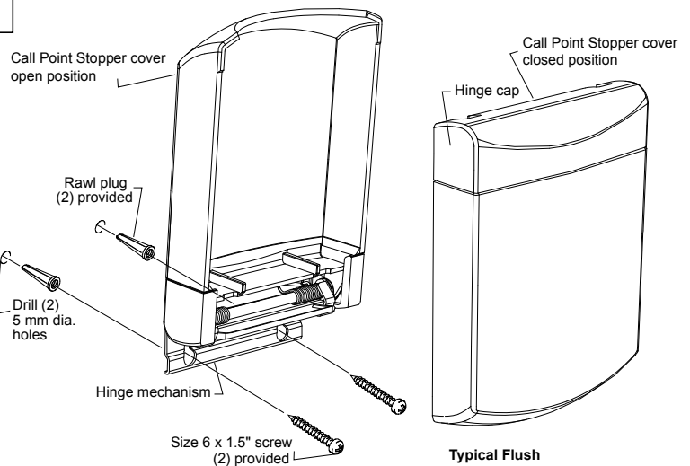
Typical Flush Installation
